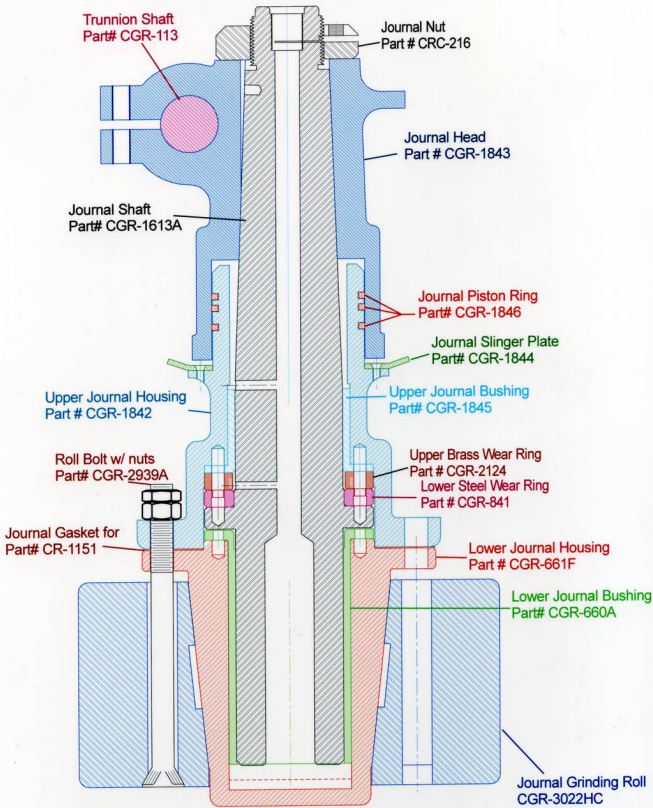
66" RM Journal Assembly
