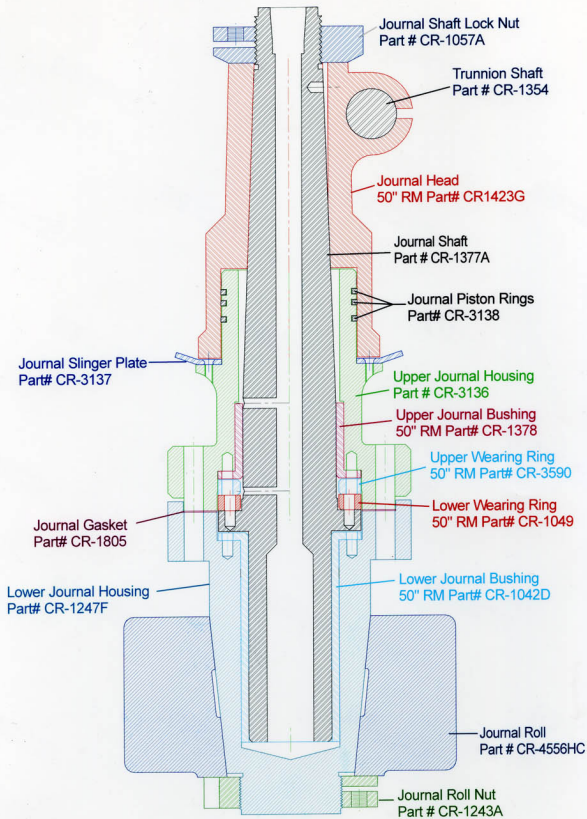
50" RM Journal Assembly
